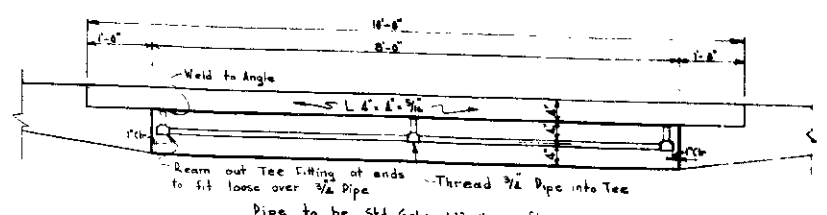
CURB WINDOW DETAIL SCALE - 1/2" = 1'
