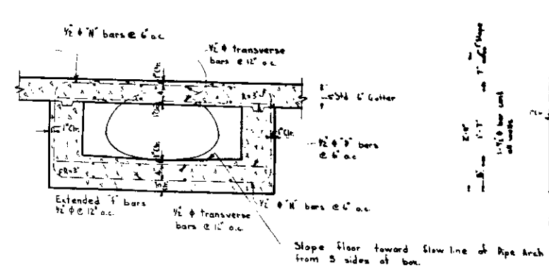
SECTION B-B SCALE - 1/2" = 1'
