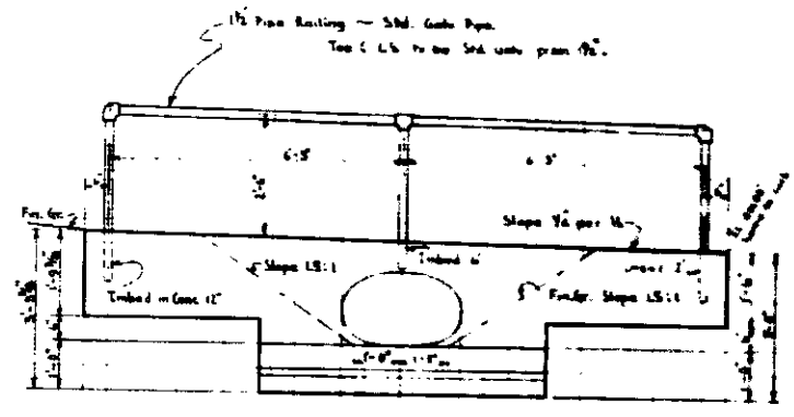
SOUTH ELEVATION - HEADWALL SCALE - 1/2" = 1'
