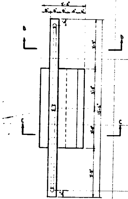
PLAN - HEADWALL SCALE - 1/2" = 1'
