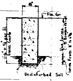
SECTION D-D SCALE - 1" = 1'
